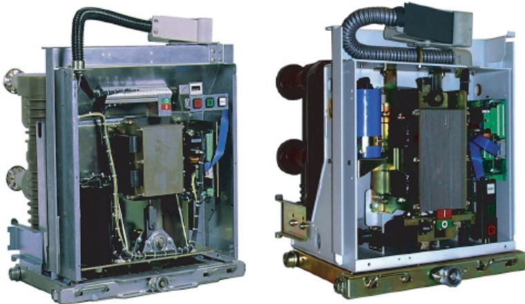
5 View of the VM1 vacuum (right) and HM1 SF 6 medium-voltage circuit-breakers showing the small number of components
